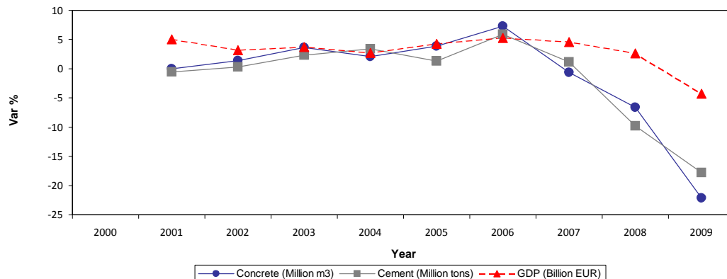
Yearly % variation 2000-2009
