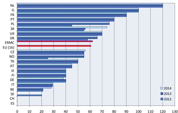
Average addition content [kg/m 3 ]
